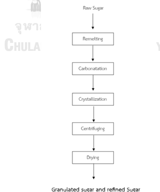
Figure 2 Granulated sugar and refined Sugar production process
