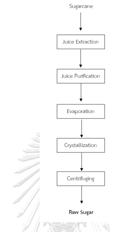
Figure 1 Raw sugar production process
