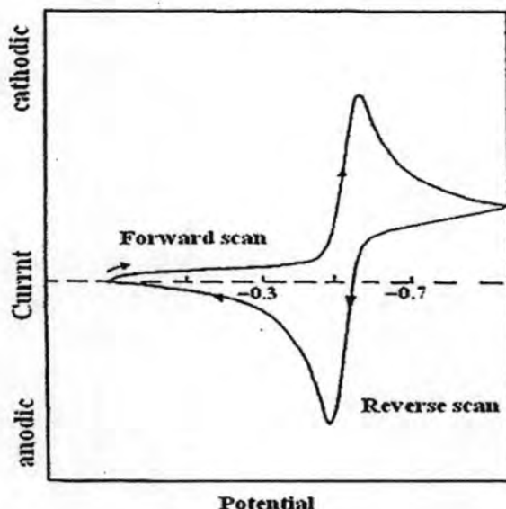
Figure 2.2 Typical cyclic voltammogram for a reversible redox process.
