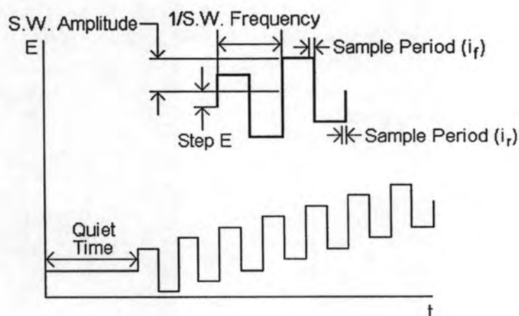
Figure 2.4 Potential-time waveform used in square wave voltammetry.
