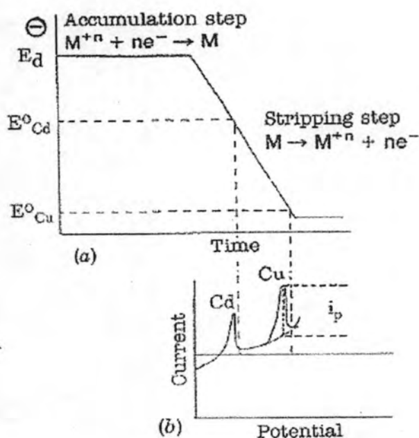
Figure 2.3 (a) Potential-time waveform and (b) stripping voltammogram of anodic stripping voltammetry.
