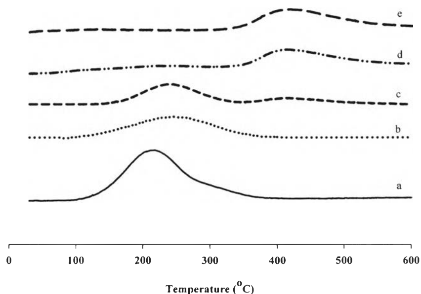
Figure 5.3 CO 2 -TPD profiles of (a) NaY, (b) 5 wt% K/NaY, (c) 10 wt% K/NaY, (d) 15 wt% K/NaY, and (e) 20 wt% K/NaY.
