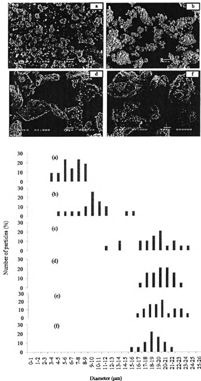
Figure 5.2 SEM images and particle size distribution of fresh catalysts: (a) NaY, (b) 5% K/NaY, (c) 10% K/NaY, (d) 15% K/NaY, and (e) 20% K/NaY; and spent catalyst: (f) 15%K/NaY.
