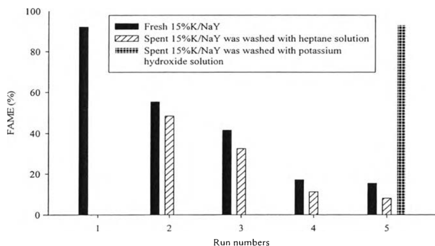
Figure 5.5 FAME (%) versus run numbers in the transesterification reaction of palm oil with methanol for the K/NaY catalyst.
