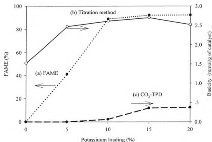
Figure 5.4 (a) FAME (%), (b) titration method, and (c) CO 2 -TPD* (only strong basicity) with varying the potassium loading.
