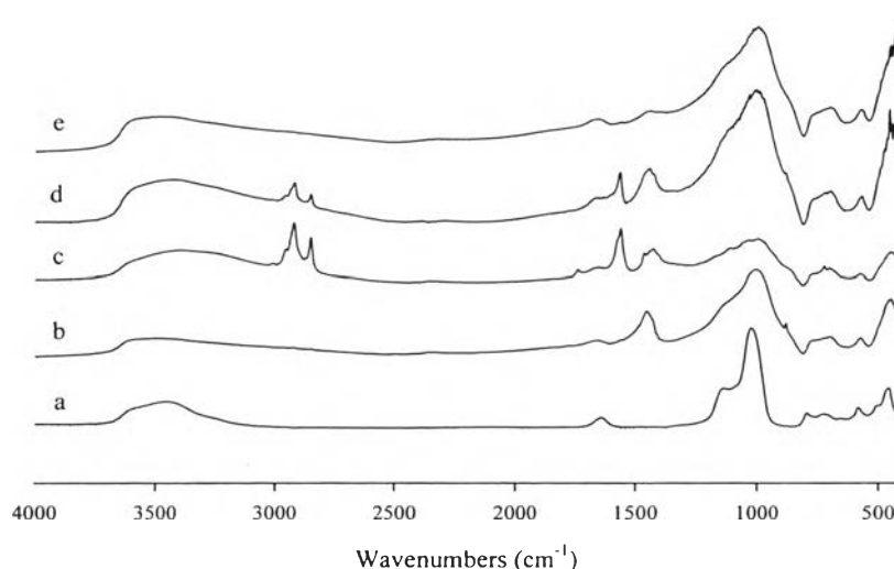
Figure 5.6 FTIR spectra of (a) NaY, (b) fresh 15wt% K/NaY, (c) spent 4 th run 15wt% K/NaY, (d) washed with heptane, and (e) washed with potassium solution of spent 4 th run 15wt% K/NaY.
