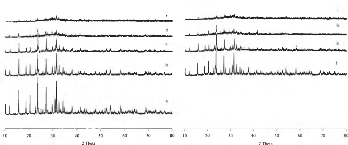
Figure 5.1 XRD patterns of the fresh catalysts: (a) NaY, (b) 5% K/NaY, (c) 10% K/NaY, (d) 15% K/NaY, and (e) 20% K/NaY; and spent catalysts: (f) 5% K/NaY, (g) 10% K/NaY, (h) 15% K/NaY, and (i) 20% K/NaY.
